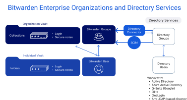
Bitwarden Enterprise Organizations and Directory Services Diagram
